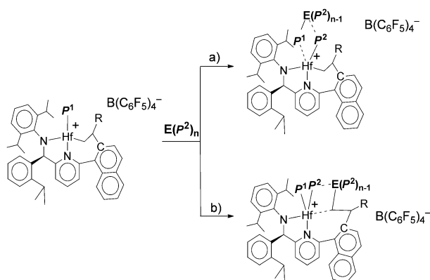
Scheme 2. Possible pathways for transalkylation in the mono-inserted active species ( P^1 and P^2 = Polymeryl chains).
