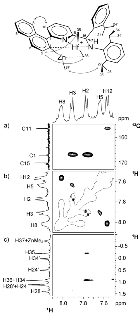
Figure 1. a) A section of the 1 H, 13 C HMBC NMR spectrum of 2 (250 K, [\text{D}_8]\text{toluene}/[\text{D}_3]\text{chlorobenzene} 1:1 v/v) showing C1/H2 and C1/H3 long-range correlations. Two sections of the 1 H ROESY NMR spectrum of 2 (250 K, [\text{D}_8]\text{toluene}/[\text{D}_3]\text{chlorobenzene} 1:1 v/v) show the H8/H12 (b) and H2/H35 (c) NOE interactions. Atom labeling relates to the sketch shown above the spectra.
